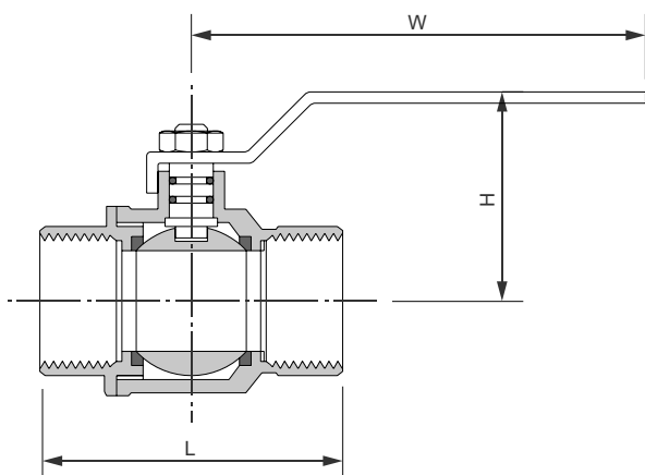
Brass F&F – SS Lever
