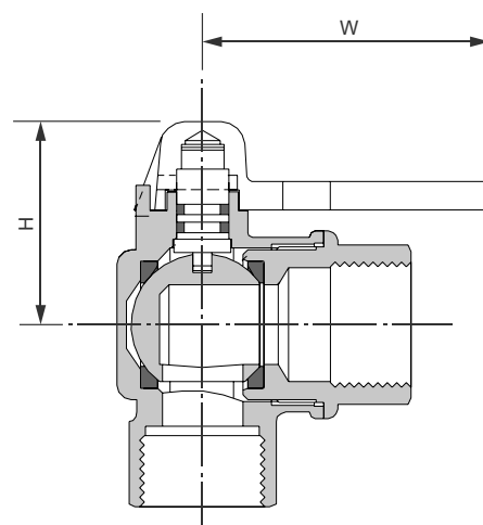
Brass R/Angle F&F – Brass Handle
