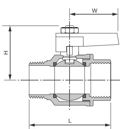
Brass M&F – Brass Handle
