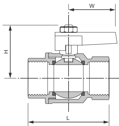
Brass F&F – Brass Handle
